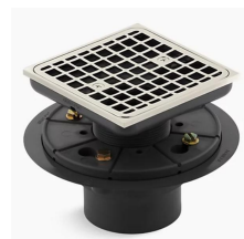
SHOWER DRAIN KOHLER- CLEARFLO FINISH: POLISHED NICKEL QTY: 1
